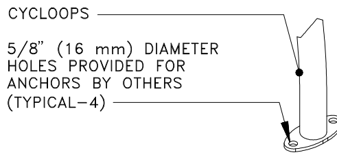
2178-84-SM (SURFACE MOUNT)
